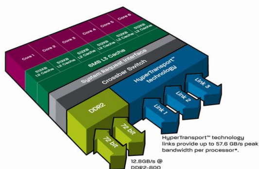
Six-Core AMD Opteron™ Processor Design 45nm for Socket F (1207) *HT3 @ up to 19.2 GB/s per link
